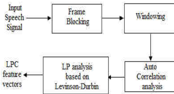
Fig.3: Block diagram of linear predictive coding
