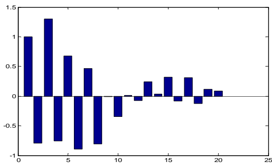
Fig.8:LPC Coefficient Feature Graph of character 'A'wav
